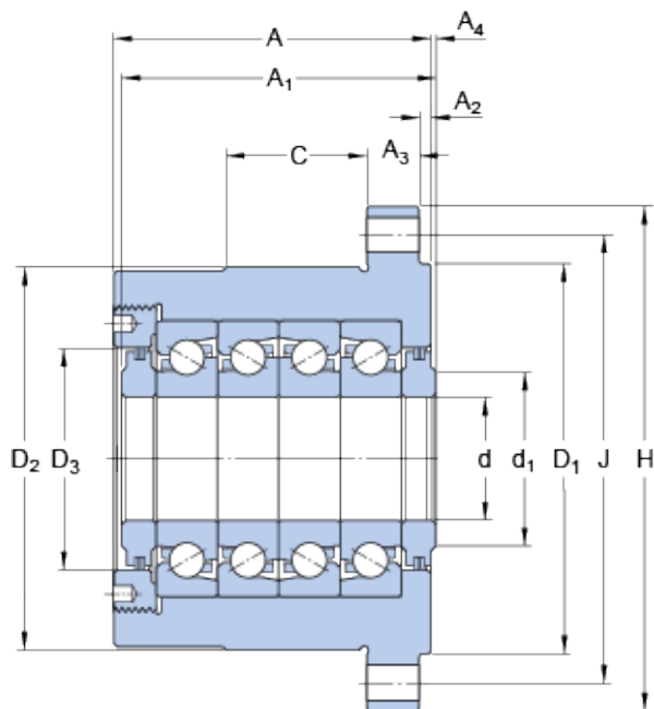
FBSA 210 A/QFC Bearing 2D drawings and 3D CAD models
